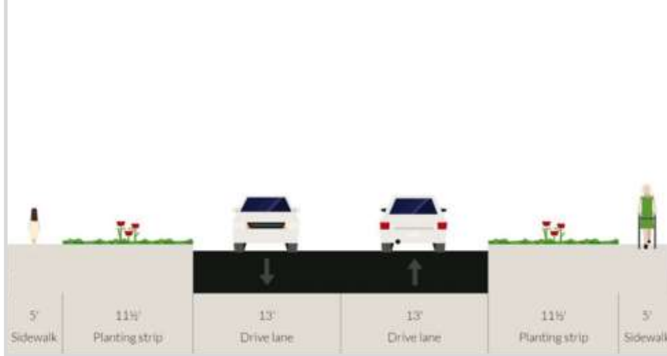
Proposed Cross Section - Neighborhood Street
